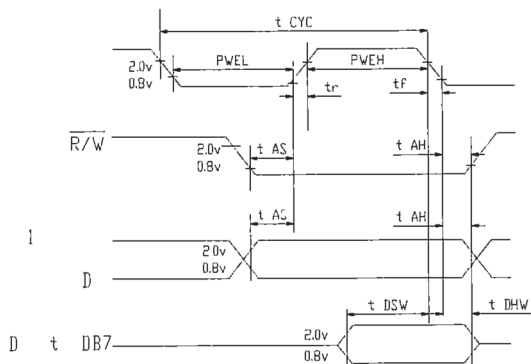
Fig1-CPU Write Timing
