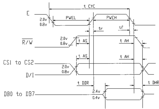
Fig2-CPU Read Timing
