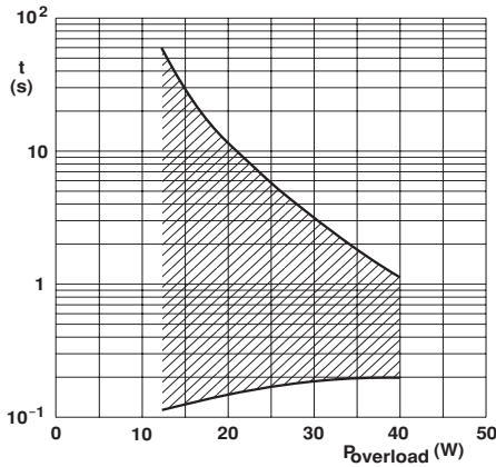
PR01 Time to interruption as a function of overload power for range: 0 R 22 \leq R_n < 1 R .
